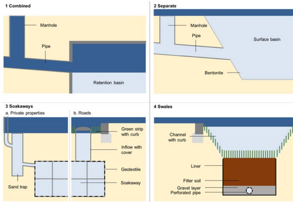
Figure 3. Schematic sketches of the elements in the four different stormwater management systems. The water level during an event with a return period of 5 (10) years is illustrated in light (dark) blue. The water level rises above surface level for events with a return period of 10 years in the systems 2-4 (Brudler et al., 2019a)
