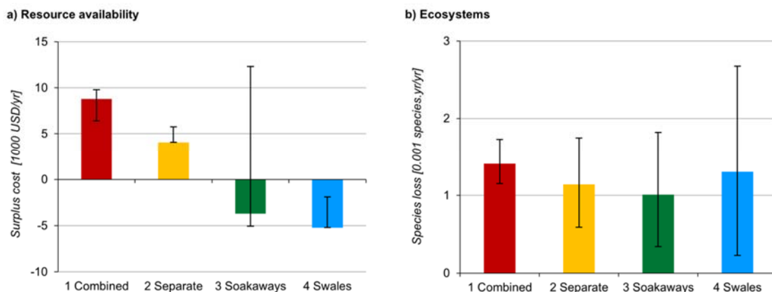
Figure 2. Damage to a) resource availability, b) ecosystems, caused by four different systems managing stormwater according to Danish flood safety and pollution management standards in a catchment area of 260ha. Negative values indicate prevented damages. Error bars illustrate the damages for a worst and best case for each system, varying both infrastructure processes and point source emissions (Brudler et al., 2019a)
